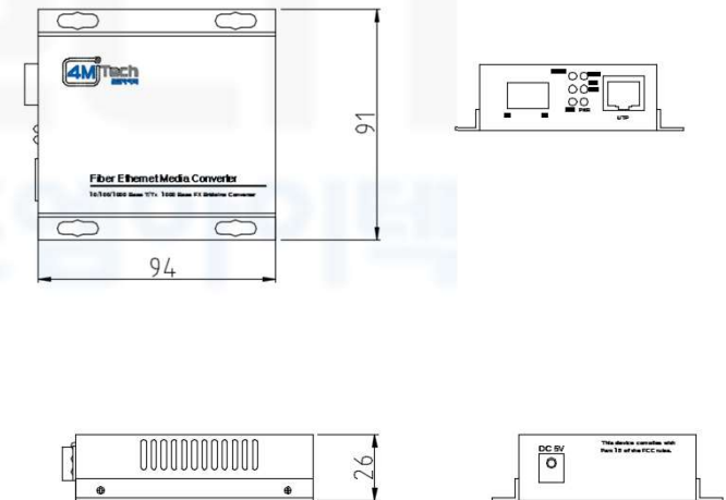
<Dimensions> W91 X D94 X H26
